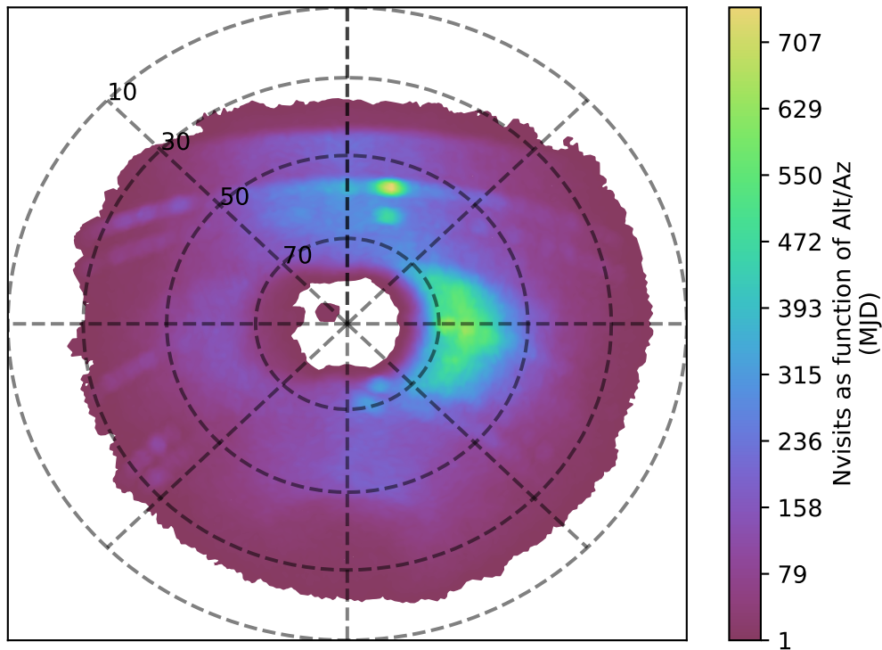
too_elab_r8_d3_griz_v3.4_10yrs u band: Nvisits as function of Alt/Az
