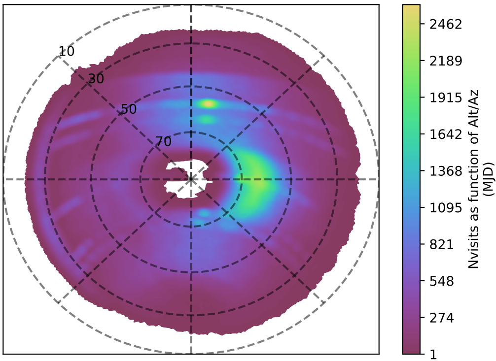
too_elab_r8_d3_griz_v3.4_10yrs r band: Nvisits as function of Alt/Az
