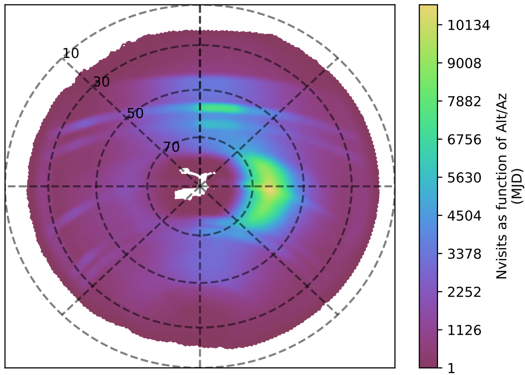
too_elab_r8_d3_griz_v3.4_10yrs all bands: Nvisits as function of Alt/Az
