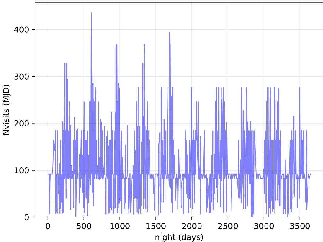
too_elab_r8_d3_griz_v3.4_10yrs DDF: Nvisits
