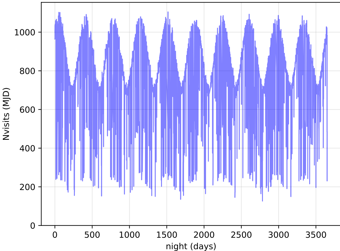
too_elab_r8_d3_griz_v3.4_10yrs All visits: Nvisits
