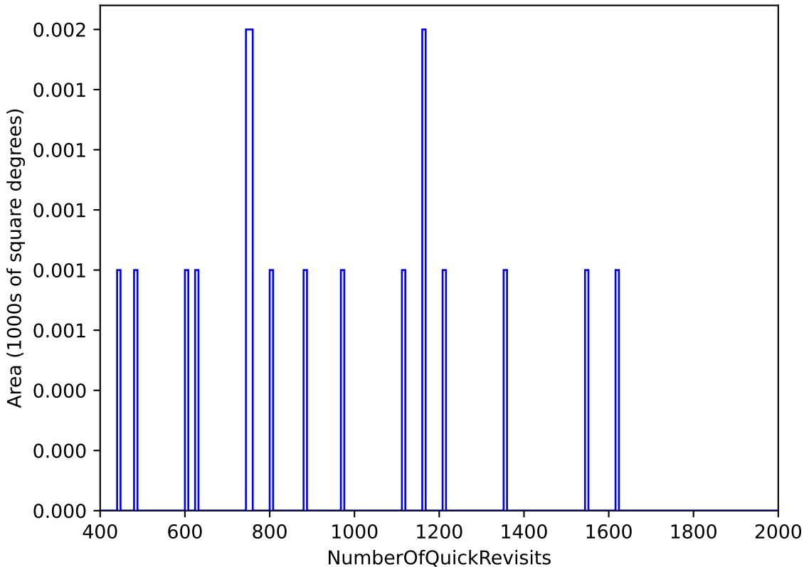
too_elab_r8_d3_griz_v3.4_10yrs WFD: NumberOfQuickRevisits
