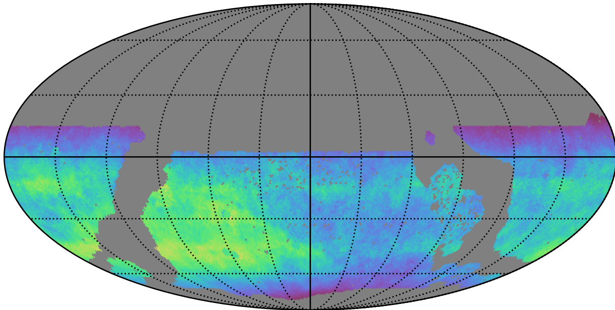
too_elab_r8_d3_griz_v3.4_10yrs WFD z band: Normalized Teff
