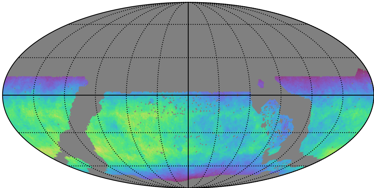
too_elab_r8_d3_griz_v3.4_10yrs WFD y band: Normalized Teff
