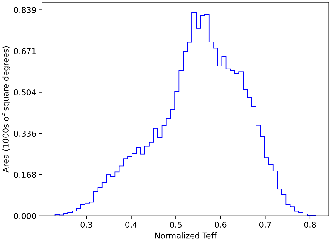
too_elab_r8_d3_griz_v3.4_10yrs WFD y band: Normalized Teff
