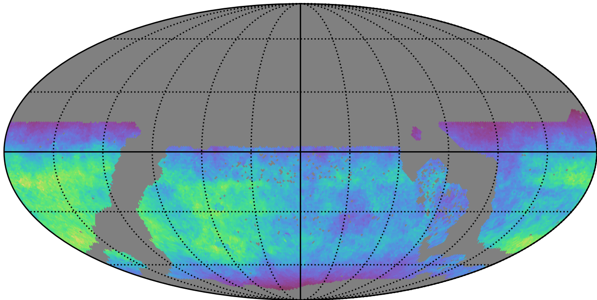
too_elab_r8_d3_griz_v3.4_10yrs WFD u band: Normalized Teff
