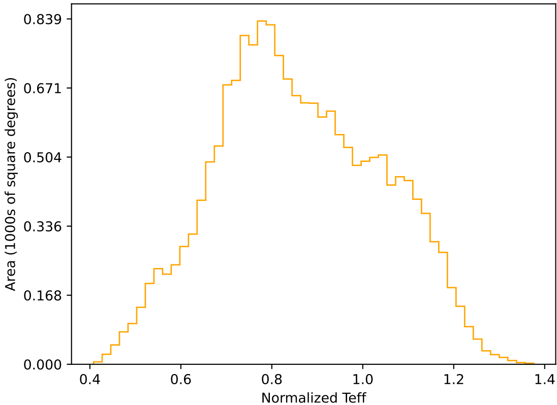
too_elab_r8_d3_griz_v3.4_10yrs WFD r band: Normalized Teff
