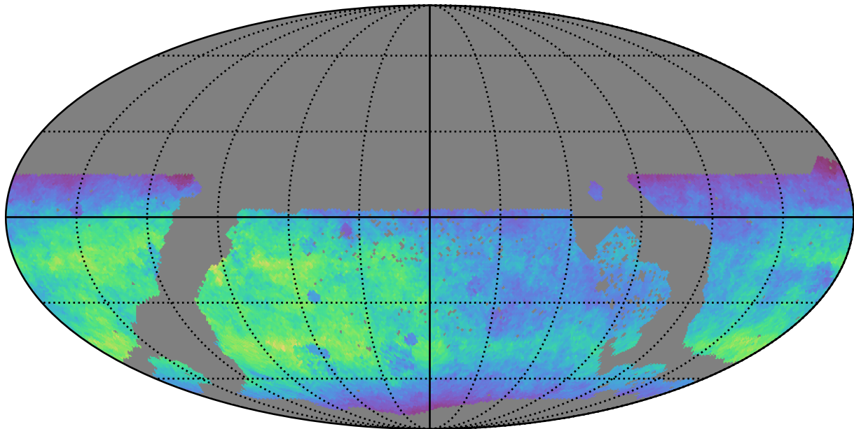
too_elab_r8_d3_griz_v3.4_10yrs WFD g band: Normalized Teff
