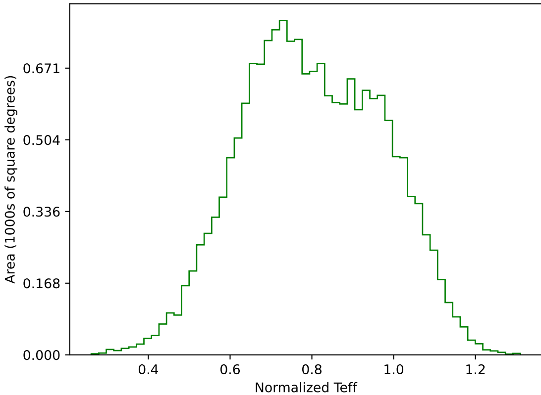
too_elab_r8_d3_griz_v3.4_10yrs WFD g band: Normalized Teff
