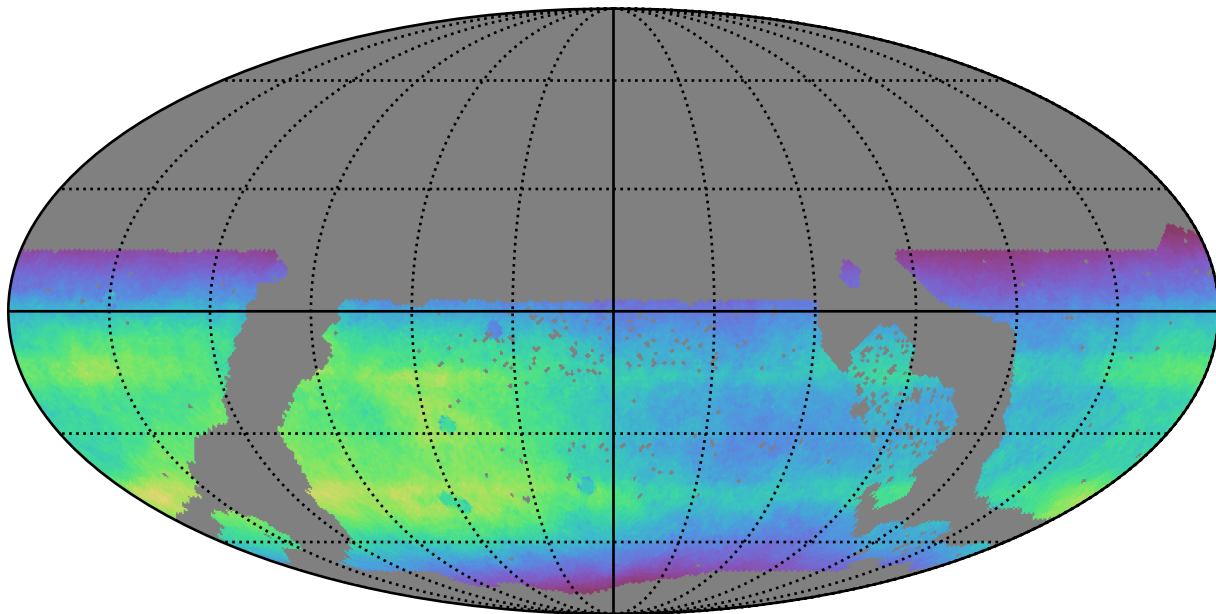
too_elab_r8_d3_griz_v3.4_10yrs WFD all bands: Normalized Teff
