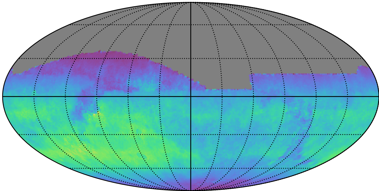
too_elab_r8_d3_griz_v3.4_10yrs All sky z band: Normalized Teff
