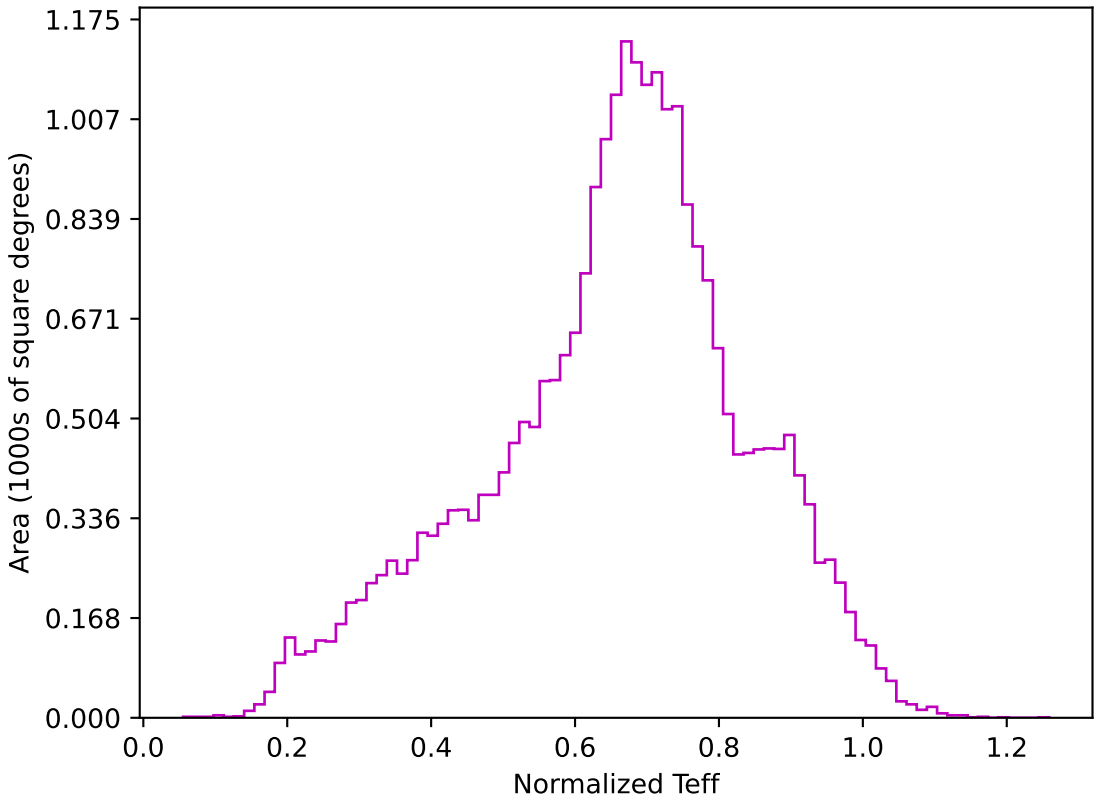
too_elab_r8_d3_griz_v3.4_10yrs All sky z band: Normalized Teff
