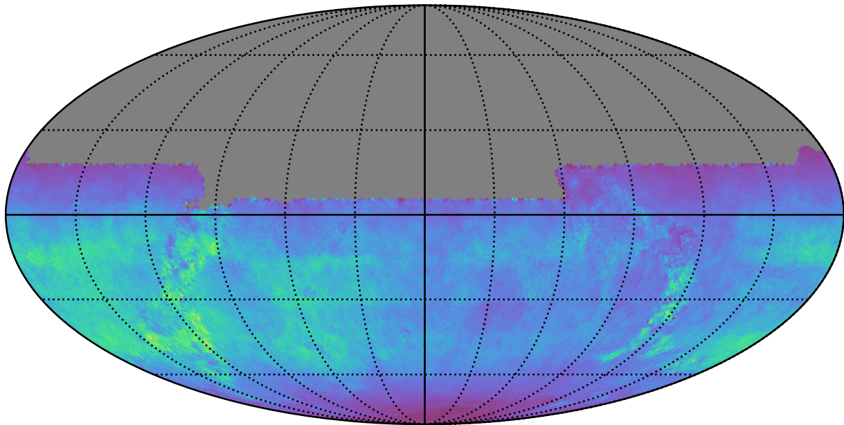
too_elab_r8_d3_griz_v3.4_10yrs All sky u band: Normalized Teff
