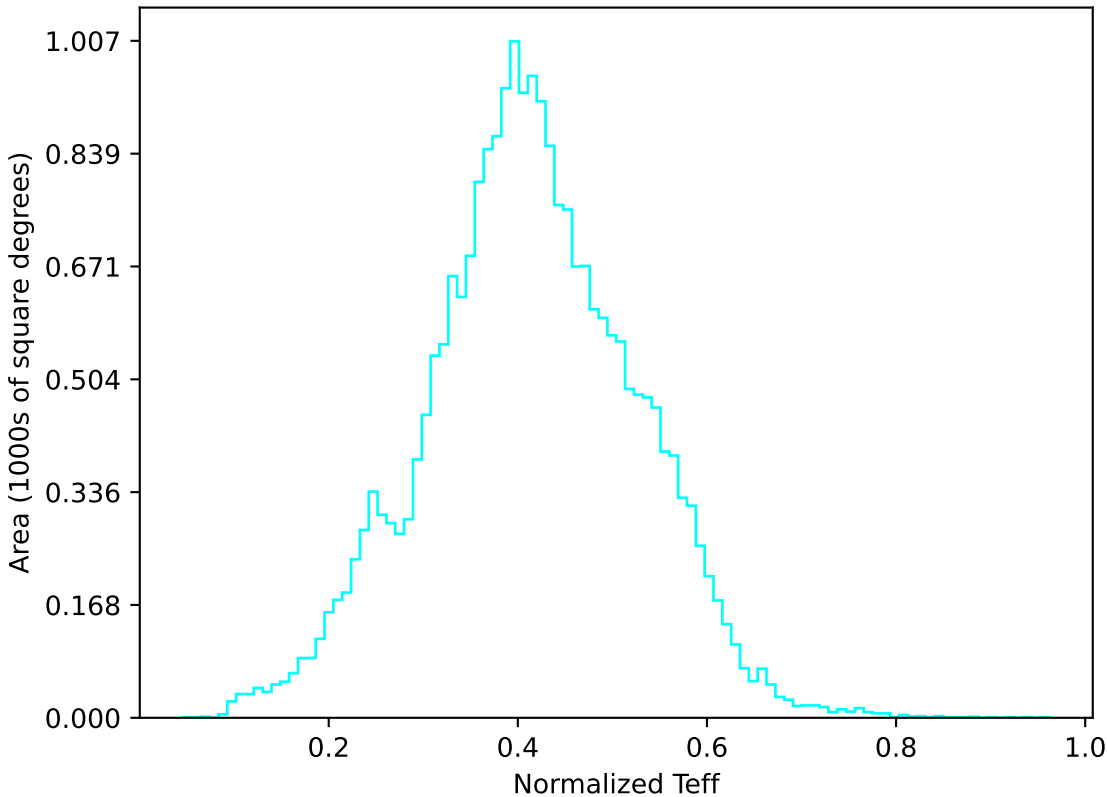
too_elab_r8_d3_griz_v3.4_10yrs All sky u band: Normalized Teff
