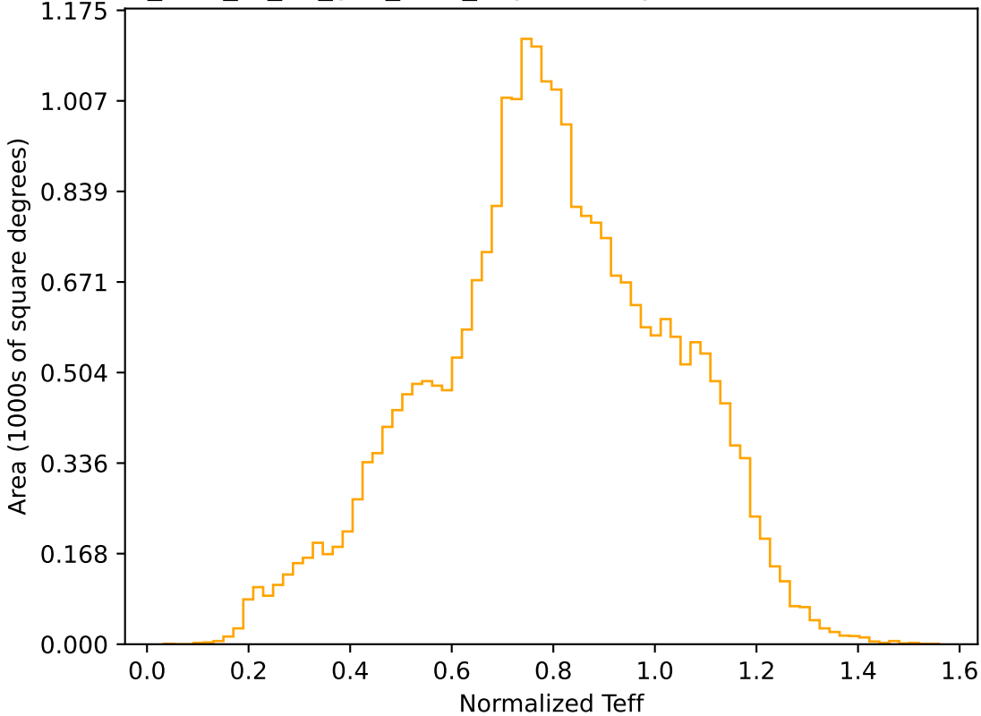
too_elab_r8_d3_griz_v3.4_10yrs All sky r band: Normalized Teff
