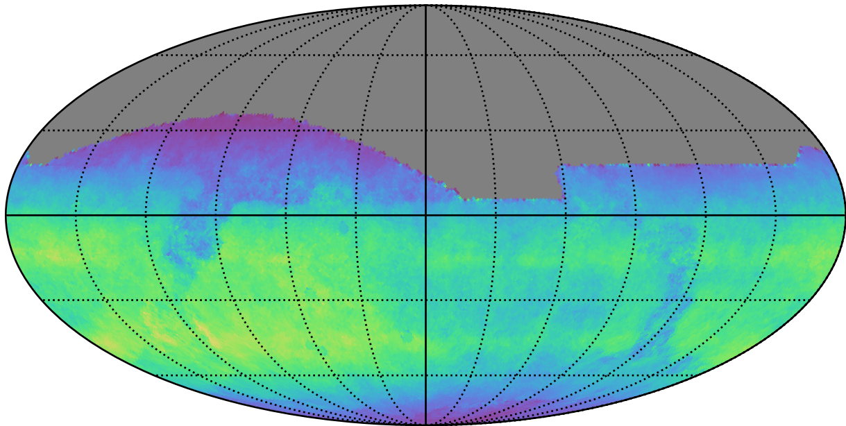
too_elab_r8_d3_griz_v3.4_10yrs All sky i band: Normalized Teff
