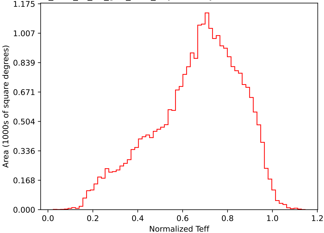
too_elab_r8_d3_griz_v3.4_10yrs All sky i band: Normalized Teff
