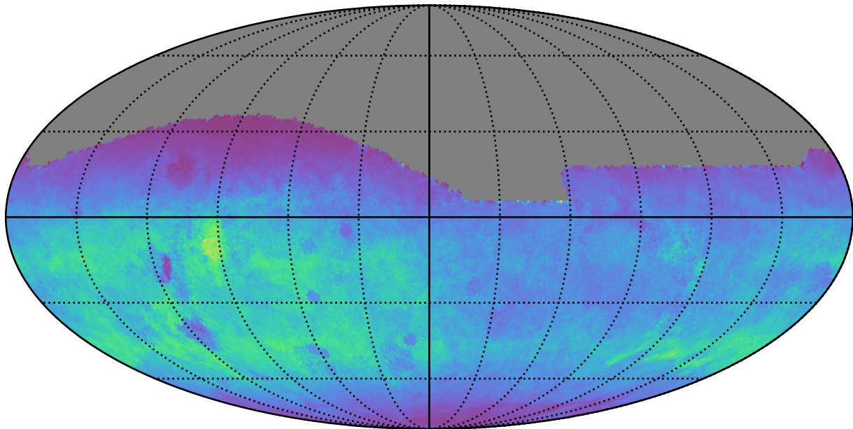
too_elab_r8_d3_griz_v3.4_10yrs All sky g band: Normalized Teff
