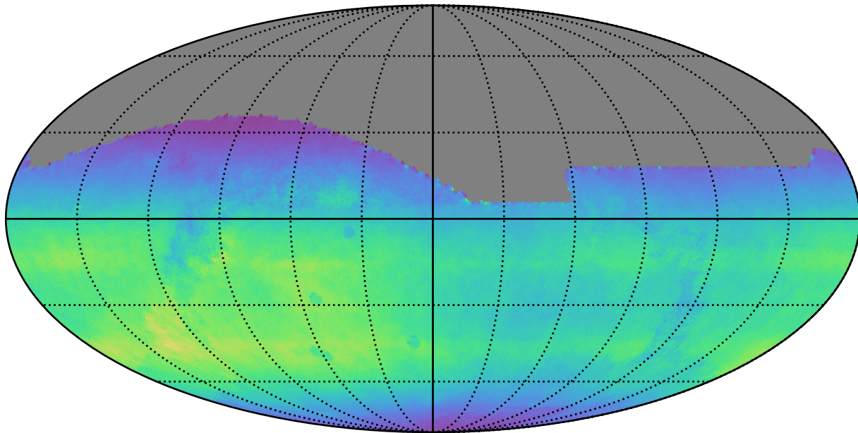
too_elab_r8_d3_griz_v3.4_10yrs All sky all bands: Normalized Teff
