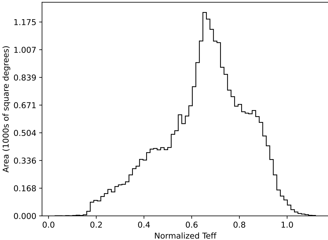
too_elab_r8_d3_griz_v3.4_10yrs All sky all bands: Normalized Teff
