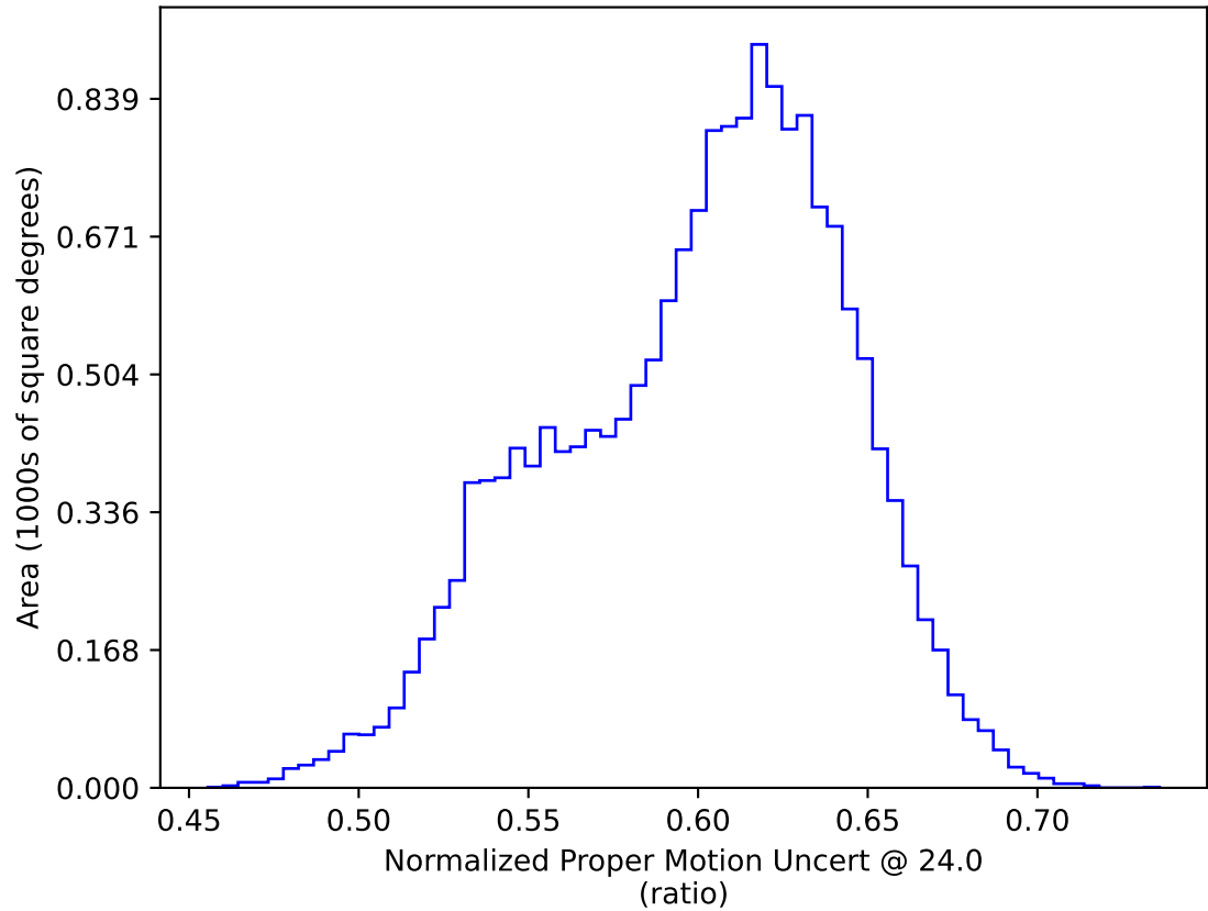
too_elab_r8_d3_griz_v3.4_10yrs WFD: Normalized Proper Motion Uncert @ 24.0
