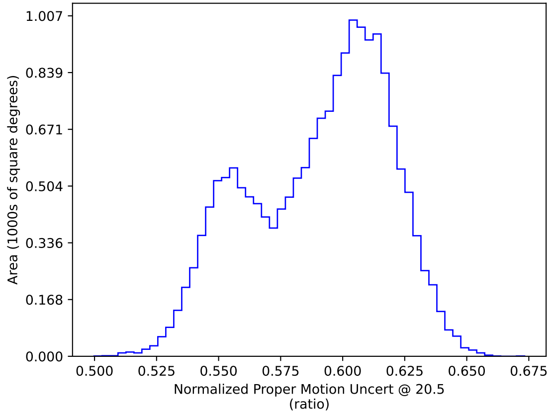
too_elab_r8_d3_griz_v3.4_10yrs WFD: Normalized Proper Motion Uncert @ 20.5
