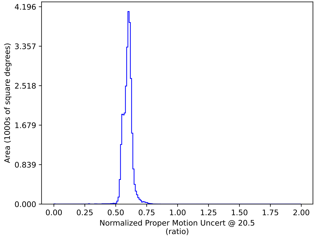
too_elab_r8_d3_griz_v3.4_10yrs All sky: Normalized Proper Motion Uncert @ 20.5
