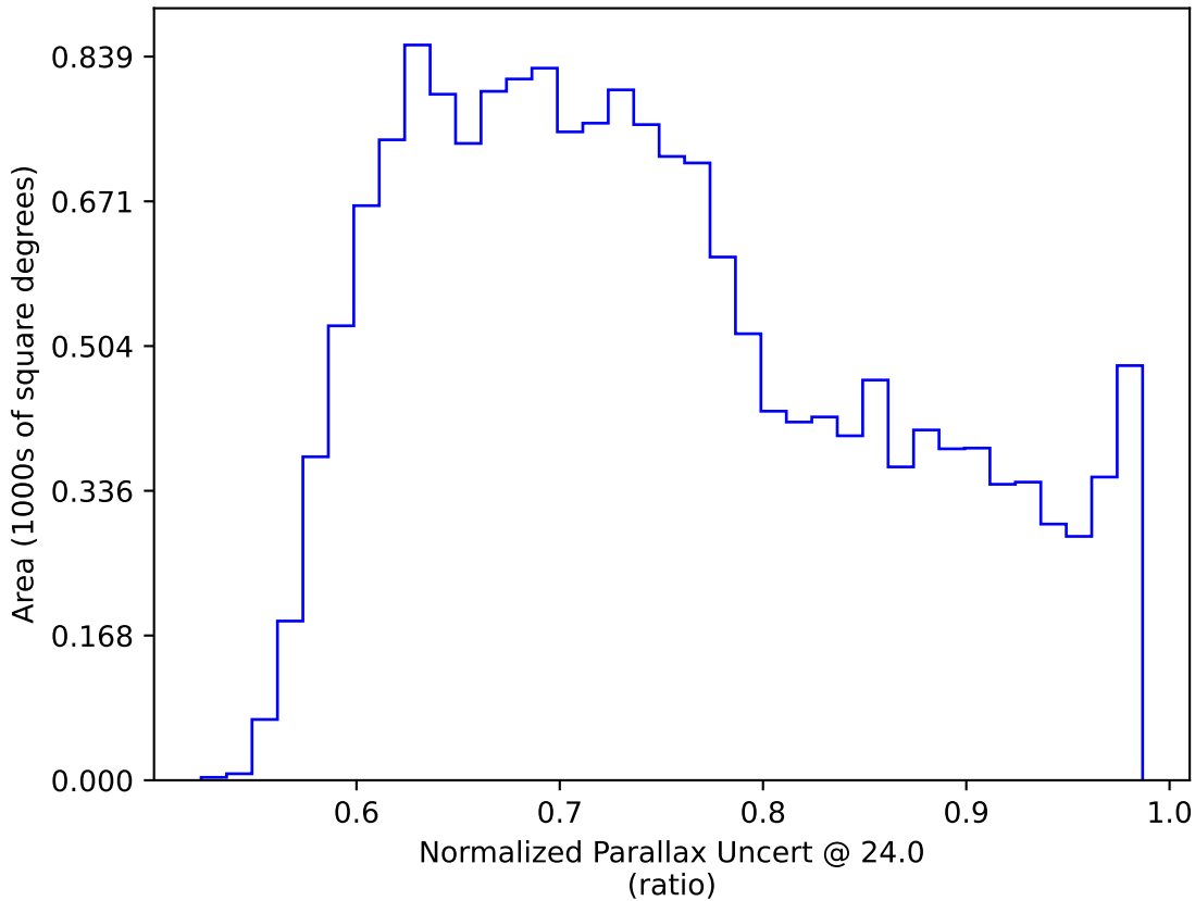
too_elab_r8_d3_griz_v3.4_10yrs WFD: Normalized Parallax Uncert @ 24.0
