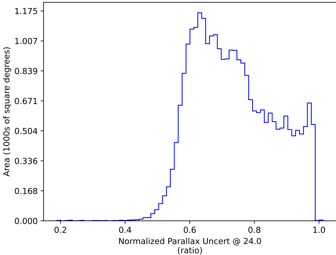
too_elab_r8_d3_griz_v3.4_10yrs All sky: Normalized Parallax Uncert @ 24.0
