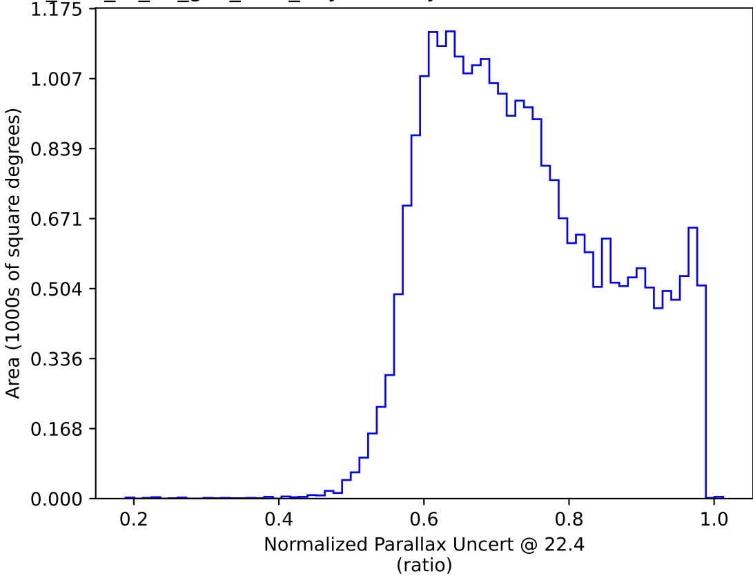
too_elab_r8_d3_griz_v3.4_10yrs All sky: Normalized Parallax Uncert @ 22.4
