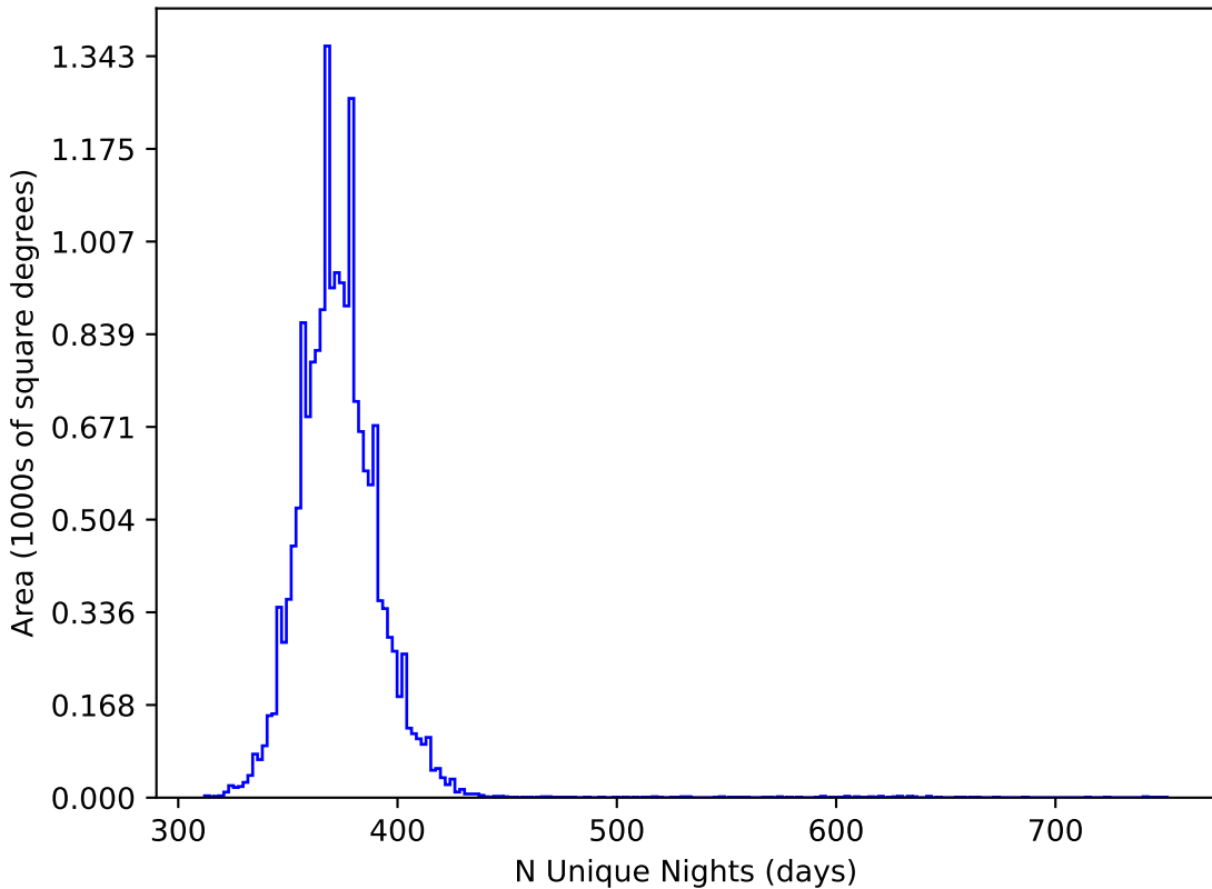
too_elab_r8_d3_griz_v3.4_10yrs WFD all bands: N Unique Nights
