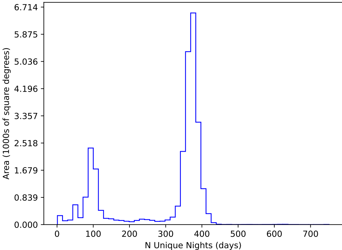
too_elab_r8_d3_griz_v3.4_10yrs All sky all bands: N Unique Nights
