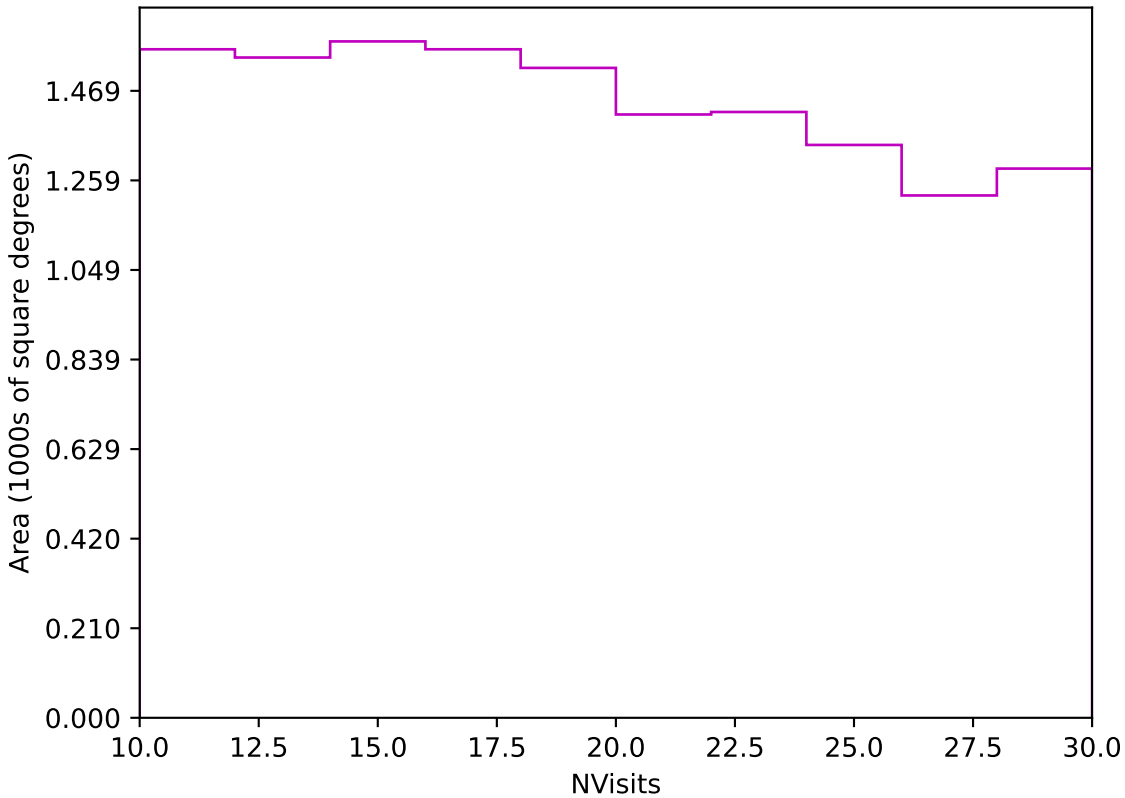
too_elab_r8_d3_griz_v3.4_10yrs Yr 3-4 z band: NVisits
