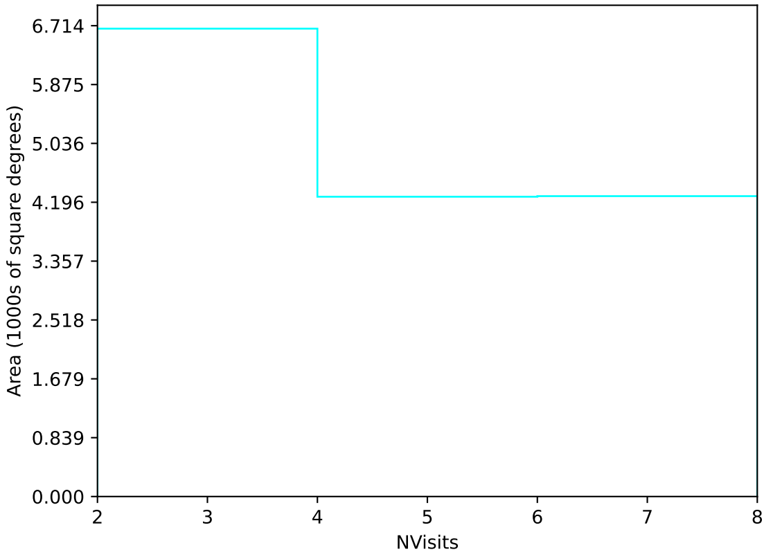
too_elab_r8_d3_griz_v3.4_10yrs Yr 3-4 u band: NVisits
