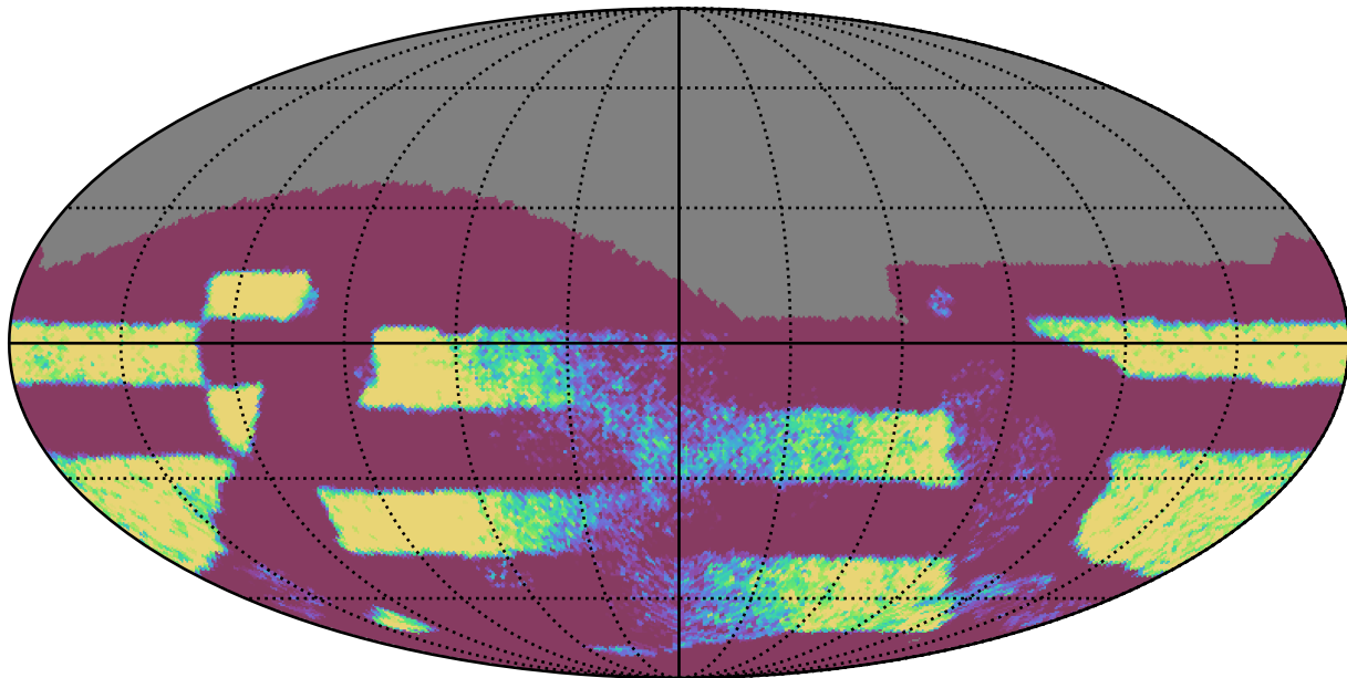
too_elab_r8_d3_griz_v3.4_10yrs Yr 3-4 all bands: NVisits
