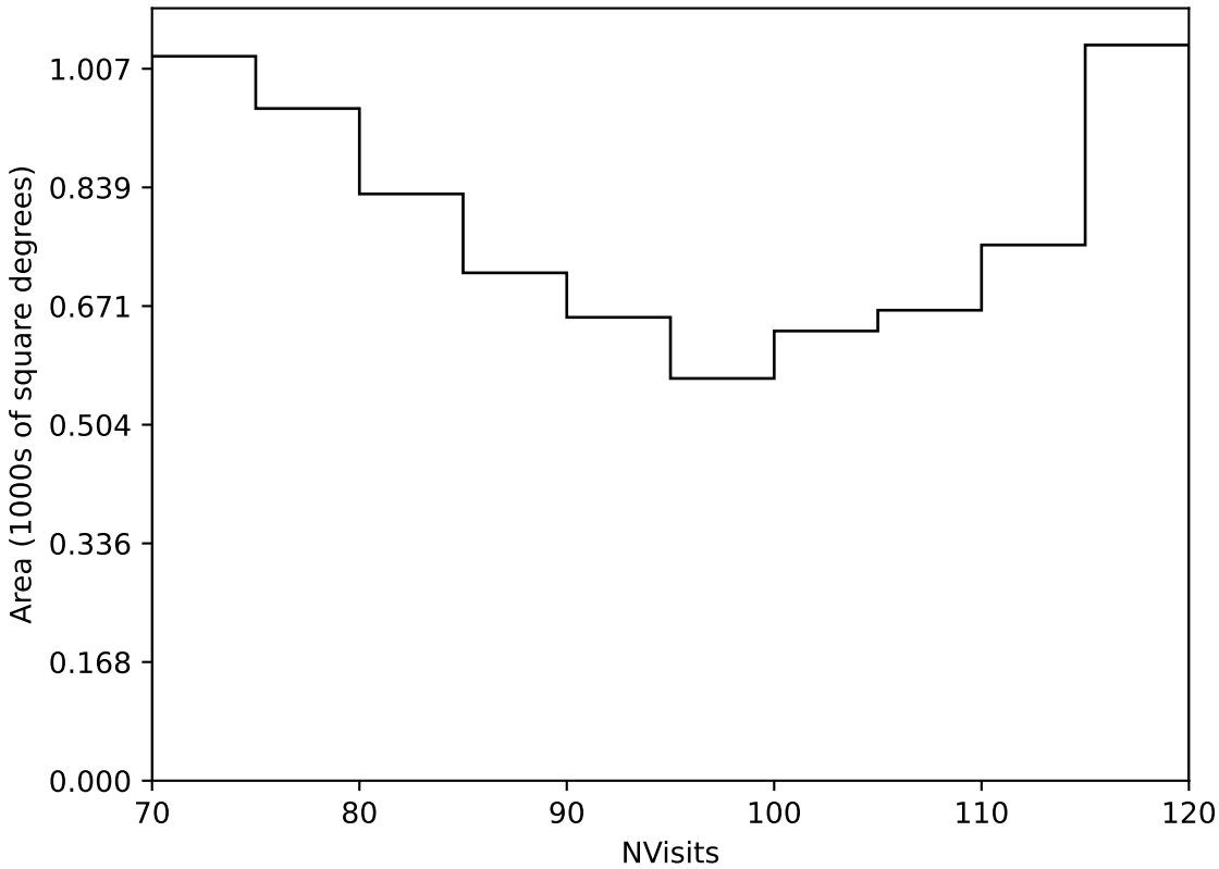
too_elab_r8_d3_griz_v3.4_10yrs Yr 3-4 all bands: NVisits
