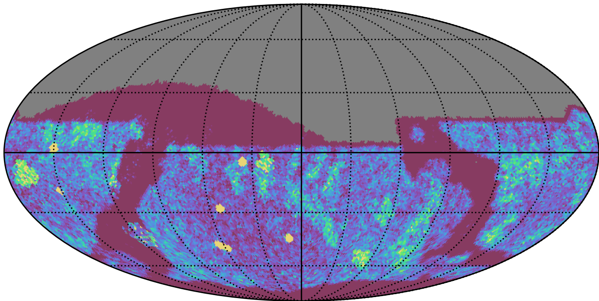
too_elab_r8_d3_griz_v3.4_10yrs Yr 1 z band: NVisits
