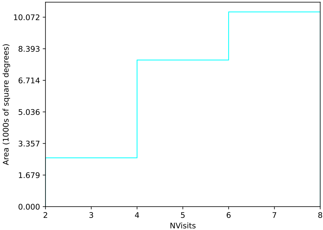
too_elab_r8_d3_griz_v3.4_10yrs Yr 1 u band: NVisits
