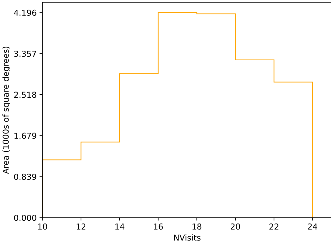
too_elab_r8_d3_griz_v3.4_10yrs Yr 1 r band: NVisits
