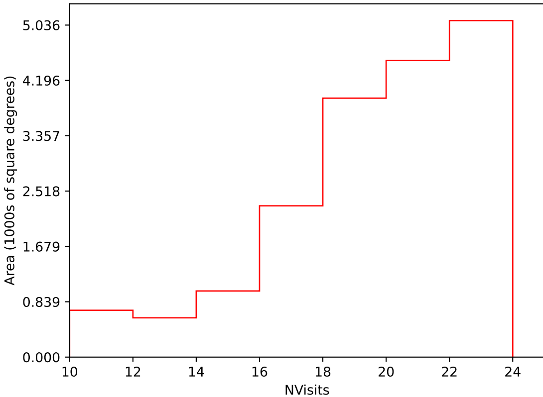
too_elab_r8_d3_griz_v3.4_10yrs Yr 1 i band: NVisits
