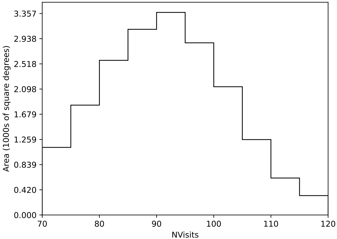
too_elab_r8_d3_griz_v3.4_10yrs Yr 1 all bands: NVisits
