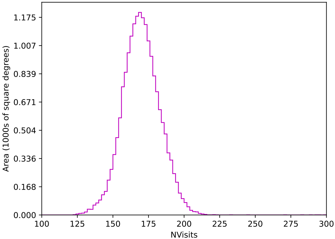
too_elab_r8_d3_griz_v3.4_10yrs WFD z band: NVisits
