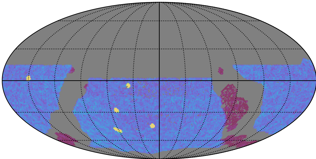
too_elab_r8_d3_griz_v3.4_10yrs WFD y band: NVisits
