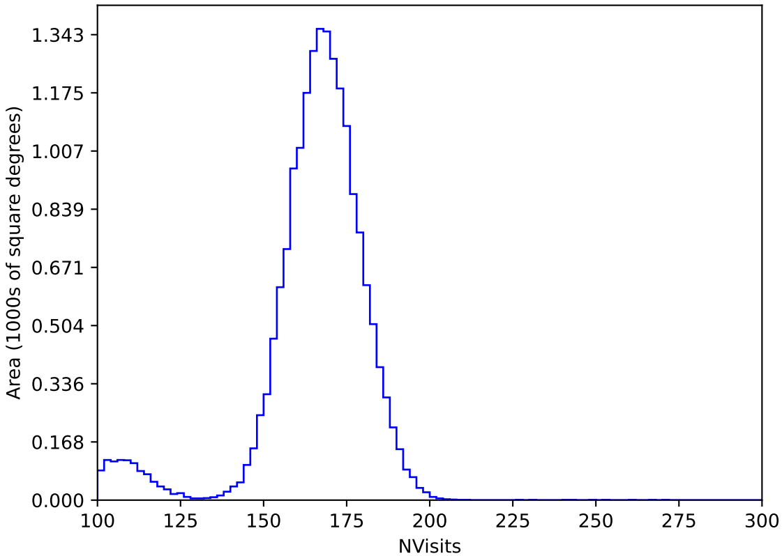
too_elab_r8_d3_griz_v3.4_10yrs WFD y band: NVisits
