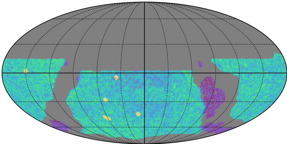
too_elab_r8_d3_griz_v3.4_10yrs WFD u band: NVisits
