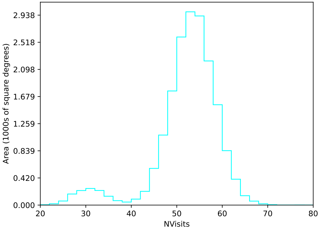
too_elab_r8_d3_griz_v3.4_10yrs WFD u band: NVisits
