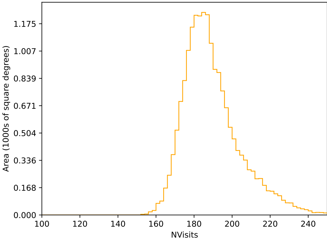
too_elab_r8_d3_griz_v3.4_10yrs WFD r band: NVisits
