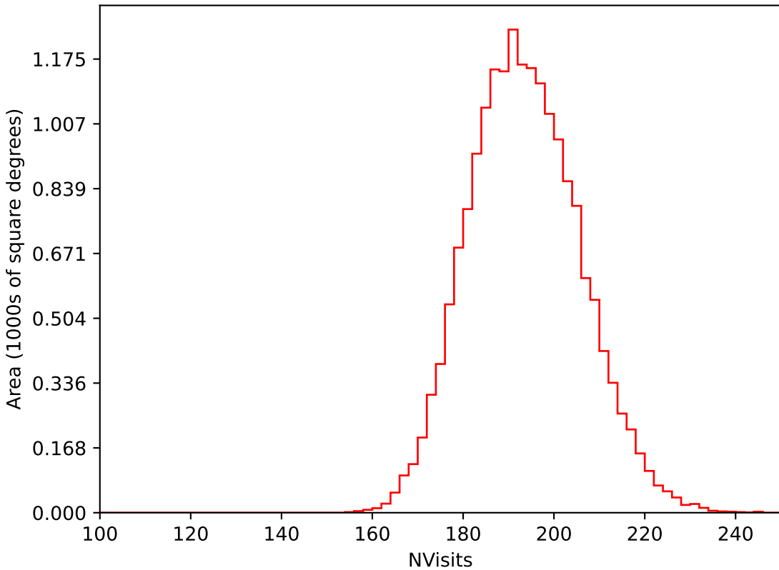
too_elab_r8_d3_griz_v3.4_10yrs WFD i band: NVisits
