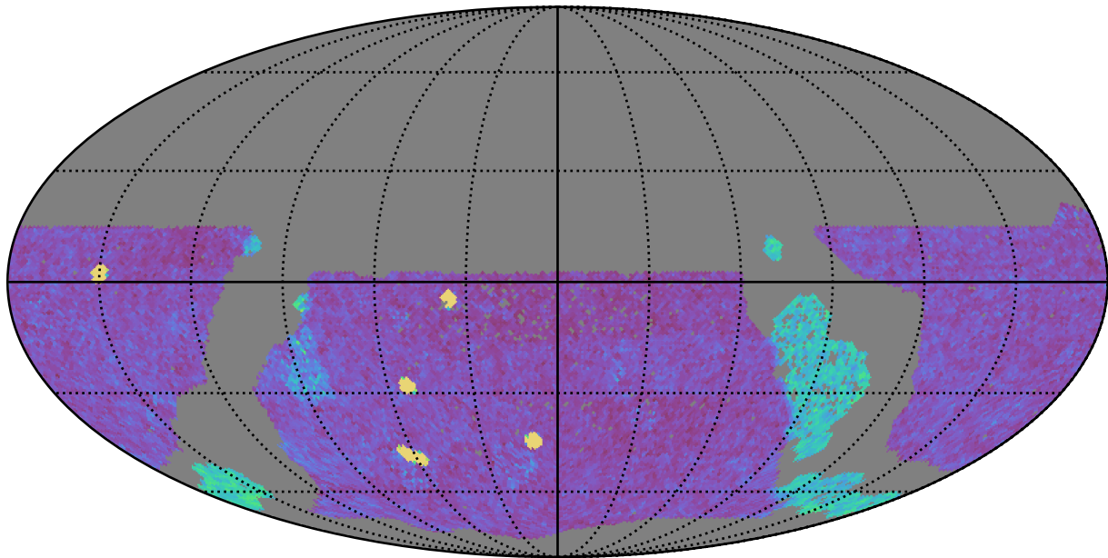
too_elab_r8_d3_griz_v3.4_10yrs WFD g band: NVisits
