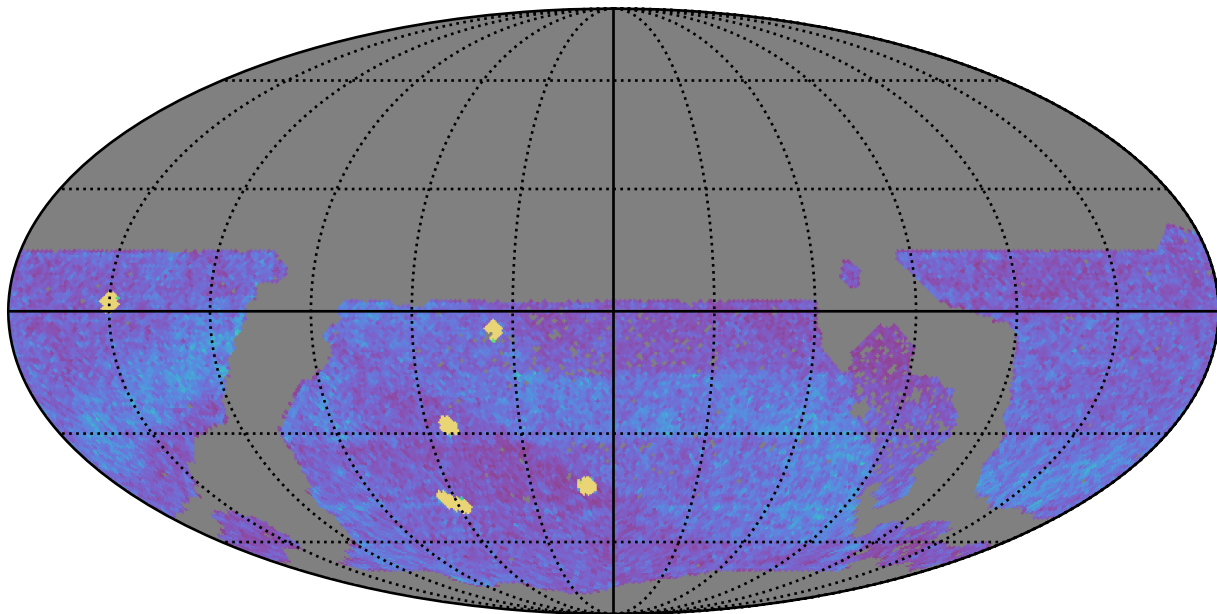
too_elab_r8_d3_griz_v3.4_10yrs WFD all bands: NVisits
